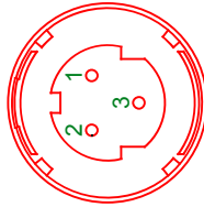
PIN VIEW HIROSE
