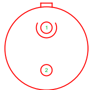
WIRE ENTRY FGG.0B.302.CLAD52Z
