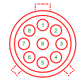
ASDD606-09PN HE PIN VIEW
