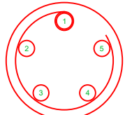
WIRE ENTRY FGG.0B.305.CLAD52Z
