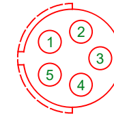
PIN VIEW
