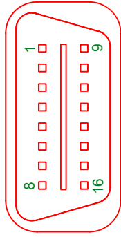
PIN VIEW
