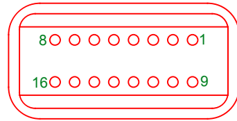
PIN VIEW
