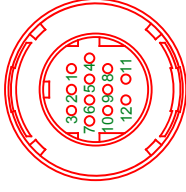
PIN VIEW HIROSE
