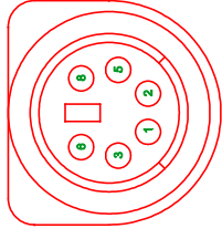
PIN VIEW
