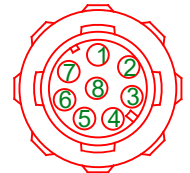
PIN VIEW 8 PIN BULGIN
