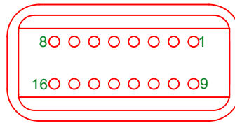
PIN VIEW
