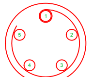
5 WAY LEMO PLUG PIN VIEW
