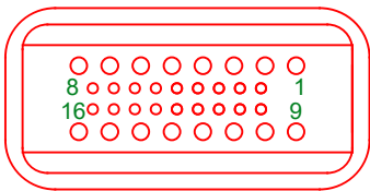
WIRE ENTRY VIEW
