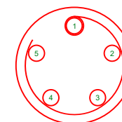
5 WAY LEMO PLUG PIN VIEW
