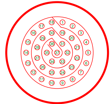
PIN VIEW
