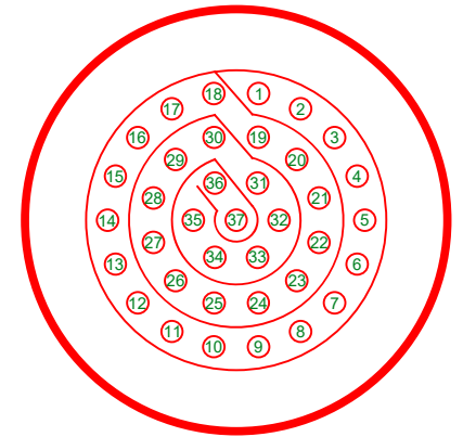
PIN VIEW
