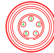
5W PLUG PIN VIEW
