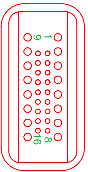
WIRE ENTRY VIEW
