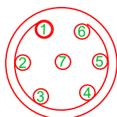
WIRE ENTRY VIEW FGG.0B.307.CLAD52Z
