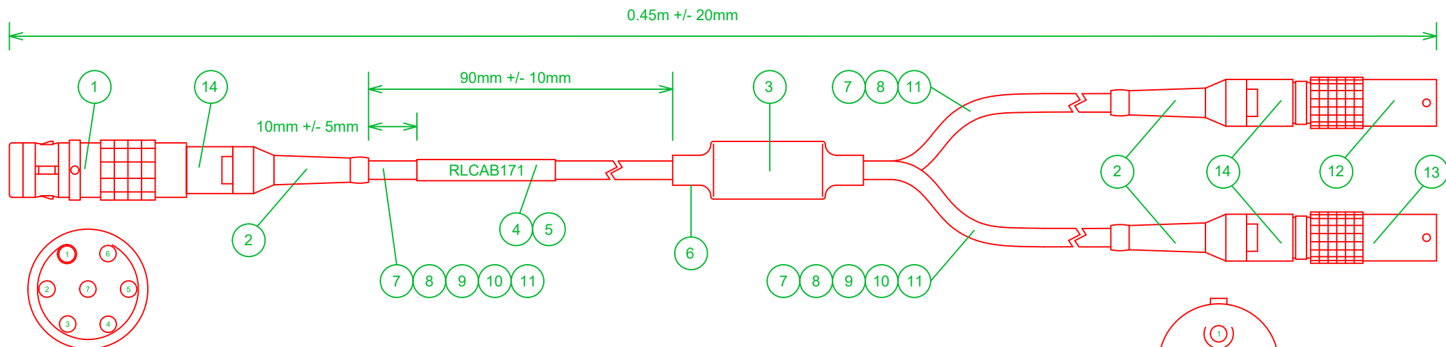
WIRE ENTRY FGG.0K.307.CLAC50Z
