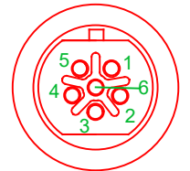
WIRE ENTRY HIROSE
